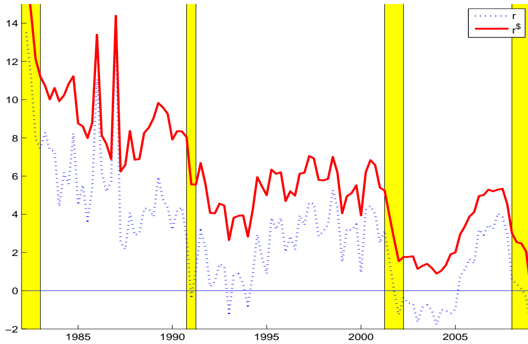
Figure 2: Real and Nominal Short Rates
